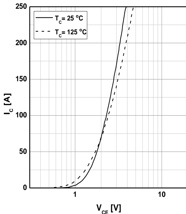
Fig2. Transfer Characteristics
