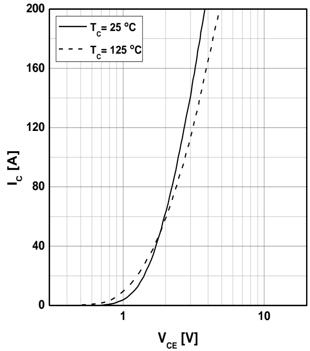
Fig2. Transfer Characteristics
